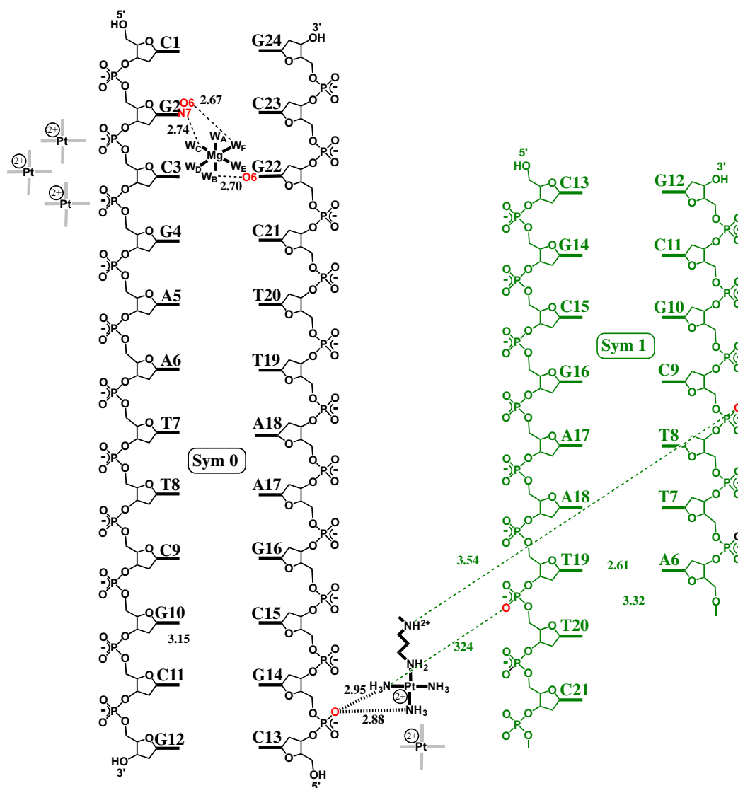
Fig. 3. Hydrogen bonding interactions of DiplatinNC-spm and hexa hydrated \text{Mg}^{2+} ion with DNA. Hydrogen bonding interactions of the phosphate clamp is indicated by bold hashed lines. Other hydrogen bonds are indicated by dashed lines. The DNA oxygen and nitrogen atoms that form hydrogen bonds are highlighted in red. Hydrogen bonding distances are given in Angstroms. Intra- and inter-symmetry hydrogen bonding network of DiplatinNC-spm with duplexes. Sym 0: x, y, z ; Sym 1: -x - 1, y + 1/2, -z + 1/2 . (For interpretation of the references to color in this figure legend, the reader is referred to the web version of this article.)
