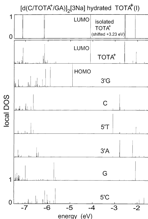
Figure 11. Local densities of states (LDOS) calculated for the isolated TOTA + (top panel) and for the hydrated TOTA + (I) 3-bp DNA segment. The LDOS of the isolated TOTA + has been rigidly shifted by 3.23 eV. In each panel we depict the weighted local DOS in the denoted region (see lettered designation in each panel). The height of a vertical bar denotes the weight of the LDOS (corresponding to the energy given on the horizontal axis) in the specified spatial region. A weight of 1 corresponds to full localization of the energy level in a particular region; for example, the HOMO level of the intercalation complex is seen to be fully localized on the 3'G and the LUMO level is fully localized on the inserted TOTA + . Note the correspondence between the (shifted) LDOS of the isolated TOTA + and that corresponding to the intercalated TOTA + (I).
