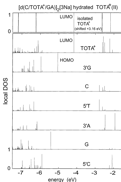
Figure 12. Local densities of states, as in Figure 11, but for the hydrated TOTA + (II) 3-bp duplex DNA segment.
