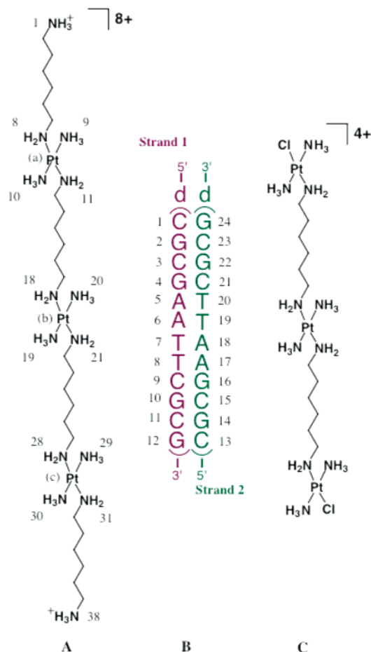
Figure 1. (A) Chemical structure of the trinuclear platinum(II) compound, TriplatinNC \{[trans\text{-Pt}(\text{NH}_3)_2(\text{NH}_2(\text{CH}_2)_6(\text{NH}_3^+))_2]_2-\mu\text{-}[trans\text{-Pt}(\text{NH}_3)_2(\text{NH}_2(\text{CH}_2)_6\text{NH}_2)_2]\}^{8+} , which was cocrystallized with DNA. (B) Double-stranded dodecamer duplex, [d(\text{CGCGAATTCGCG})]_2 (DDD), used for this crystallographic study. (C) For comparison, a cross-linking trinuclear platinum(II) complex, \{[trans\text{-Pt}(\text{NH}_3)_2\text{Cl}]_2-\mu\text{-}[trans\text{-Pt}(\text{NH}_3)_2(\text{NH}_2(\text{CH}_2)_6\text{NH}_2)_2]\}^{4+} (BBR3464), with labile chloride ligands.
