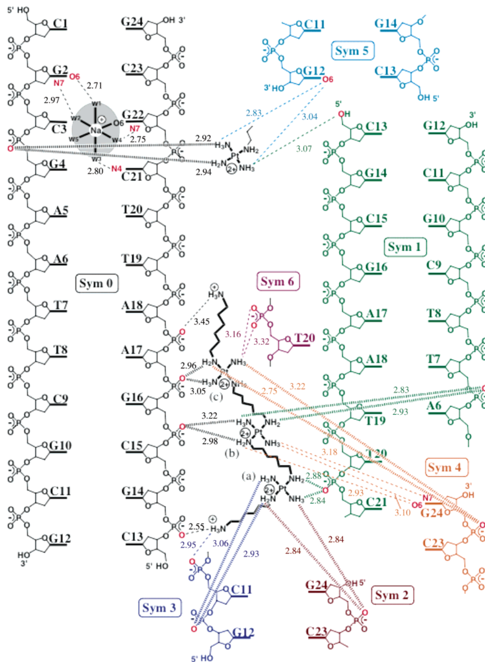
Figure 3. Hydrogen bonding interactions of TriplatinNC with DNA. Hydrogen bonding interactions of Phosphate Clamps are indicated by bold hashed lines. Other hydrogen bonds are indicated by dashed lines. TriplatinNC a forms seven Phosphate Clamps. The discernible portion of TriplatinNC b forms one Phosphate Clamp. A Na + ion (shaded) interacts directly with the O6 of a guanine and with five water molecules. Oxygen and nitrogen atoms that form hydrogen bonds with TriplatinNC or the Na + are highlighted in red. Hydrogen bonding distances are given in Angstroms. Interactions involving symmetry-related molecules are color-coded. The symmetry operators are as follows: Sym 0: x, y, z ; Sym 1: -x - 1, y + 1/2, -z + 1/2 ; Sym 2: -x - 1/2, -y + 1, z - 1/2 ; Sym 3: x + 1, y, z ; Sym 4: -x - 3/2, y + 1, z - 1/2 ; Sym 5: -x - 3/2, -y + 1, z + 1/2 ; Sym 6: -x - 3/2, -y + 1, z + 1/2 .
