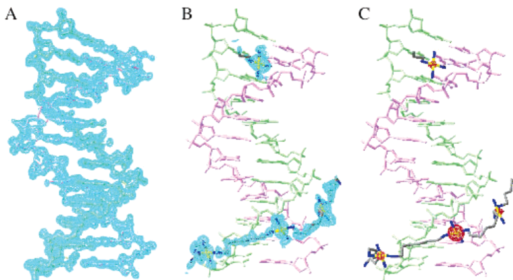
Figure 2. Electron density maps of the TriplatinNC–DNA complex. Both TriplatinNC a and TriplatinNC b are shown. (A) Sum electron density surrounding the DNA, contoured at 1.5 \sigma . TriplatinNC a and TriplatinNC b are omitted for clarity. (B) Sum ( 2F_o - F_c ) electron density surrounding TriplatinNC a and TriplatinNC b , contoured at 0.9 \sigma . (C) Anomalous electron density contoured at 5 \sigma . The positions of the Pt(II) atoms are indicated by the anomalous peaks.
